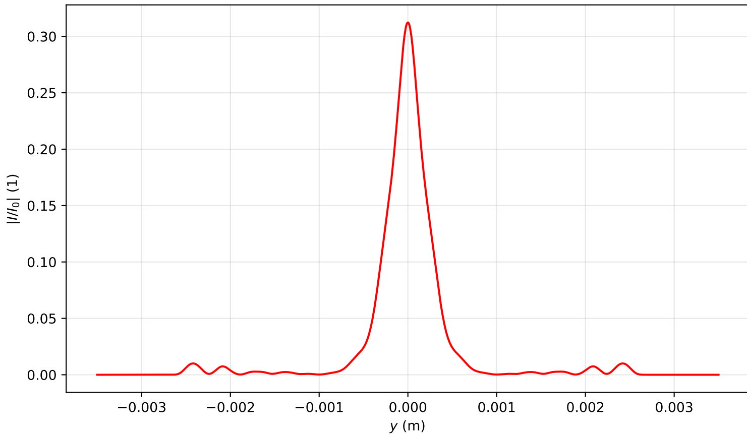
Intensity profile I(x = 0, y, z = 2.229)/I_0 , P_{in}=6.0P_{cr} , artificial time
